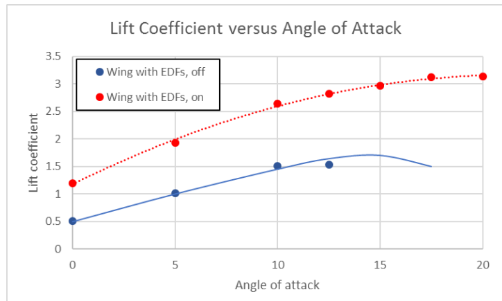
Figure 2: Lift curve
