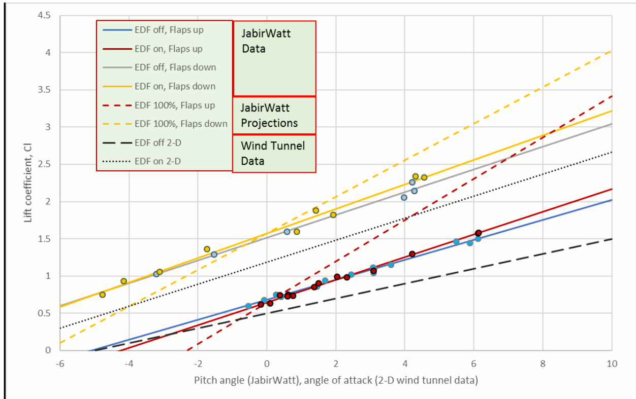
Figure 3: Lift Coefficient Comparisons based on JabirWatt inflight data
